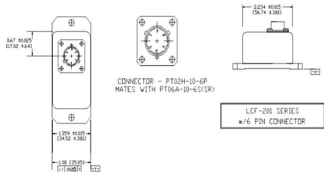
Pin Out: LCF-200 Series Accelerometer
