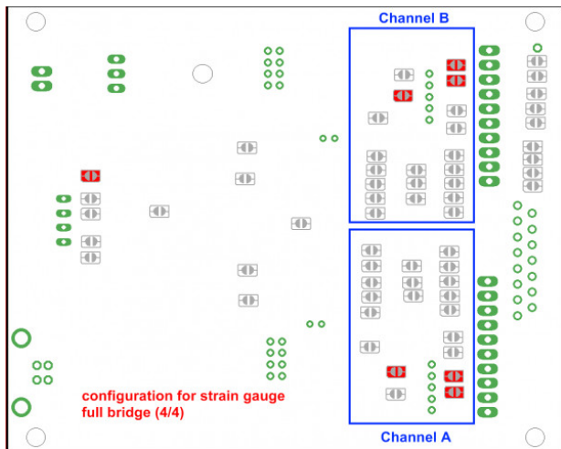
Figure 5: strain gauge full bridges
