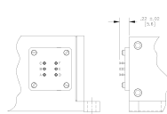
Pin-Terminal Version
